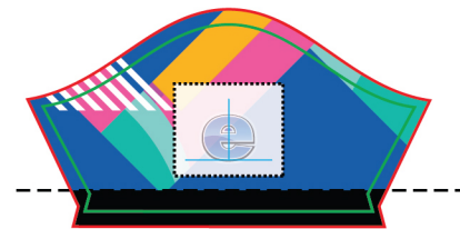
S.SLEEVE RIGHT
